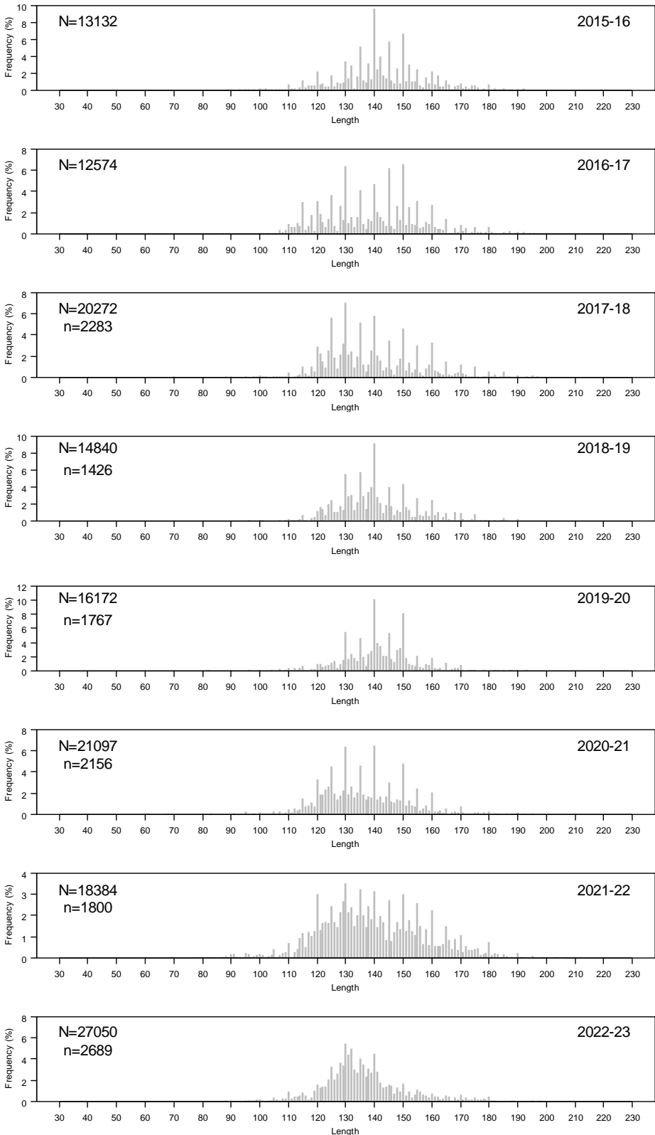
Figure 5 Length frequency histograms for retained SBT longline catch in Australian waters raised to total catch, 2015–16 to 2022–23 quota years
