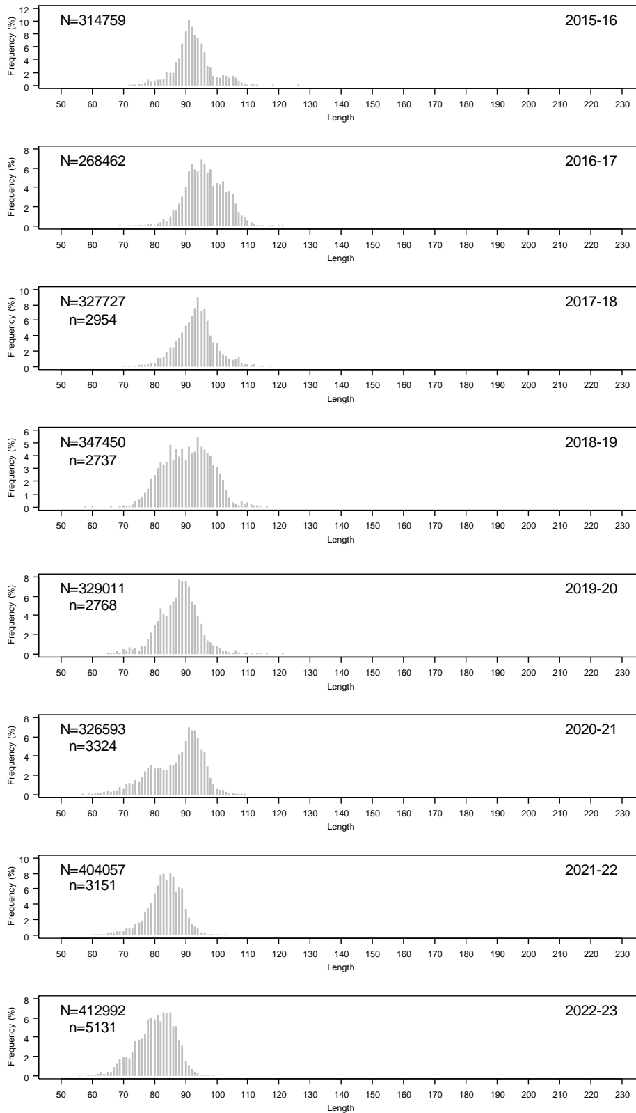
Figure 4 Length frequency of SBT purse seine catch in Australian waters raised to total catch, 2015–16 to 2022–23 fishing seasons
