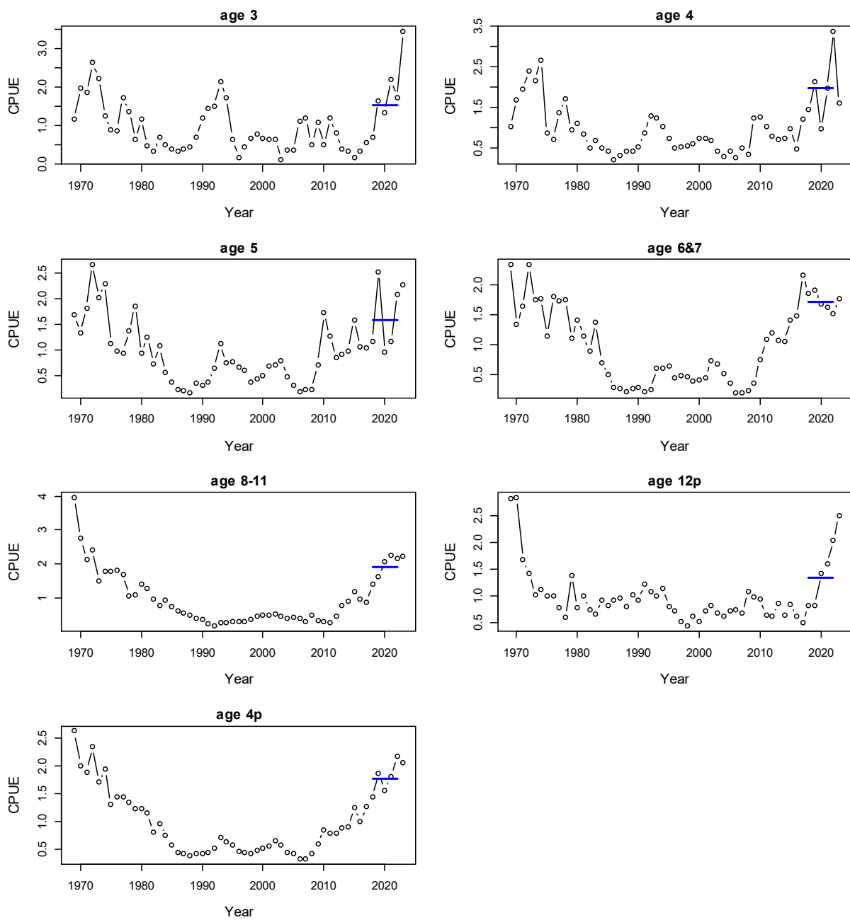
Fig. 1-1. Nominal CPUE of Japanese longline fishery by age groups. The horizontal lines indicate the past 5-year averages over 2018-22.
