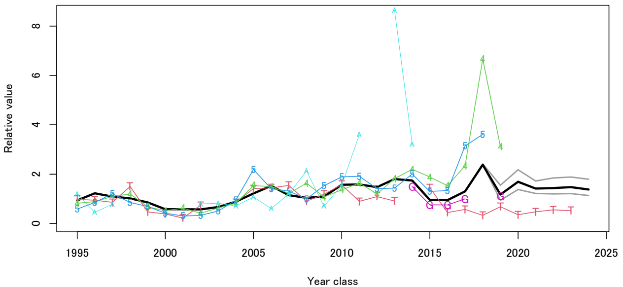
Fig. 3-2. Comparison of relative historical trends of various SBT recruitment indicators including recruitment estimates from the OM. A: aerial survey index, G: age 2 SBT absolute abundance estimated from gene-tagging, T: grid-type trolling index, 4 and 5: standardized Japanese longline CPUE index for age 4 and 5 SBT, black and grey solid lines: median recruitment (with an 80% probability envelope) estimated from stock assessment using the OM.
