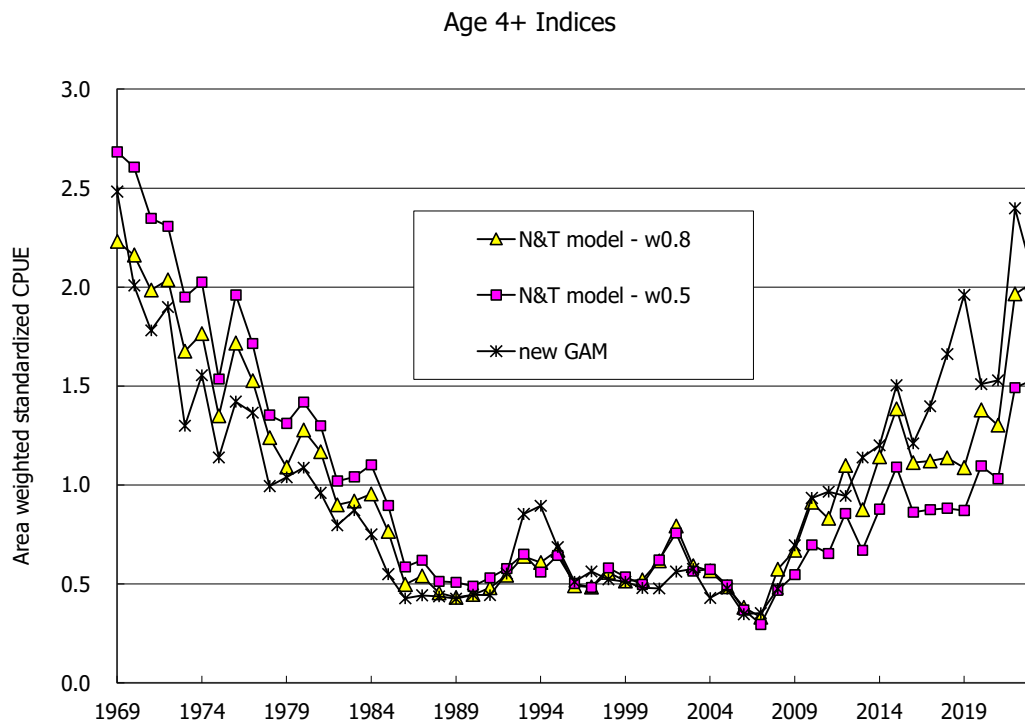
Fig. 1-6. Trends of various abundance indices for age 4+: Nishida & Tsuji model with all vessels data; new GAM series with all vessels data.
