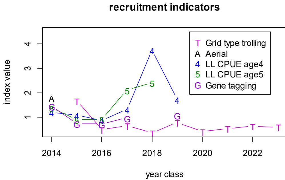
Fig. 5-1. Trends of recruitment in recent years. Note that the x-axis is year class, and the aerial survey (AS) index was plotted assuming that the AS index primarily represented the trend of age 3 SBT.
