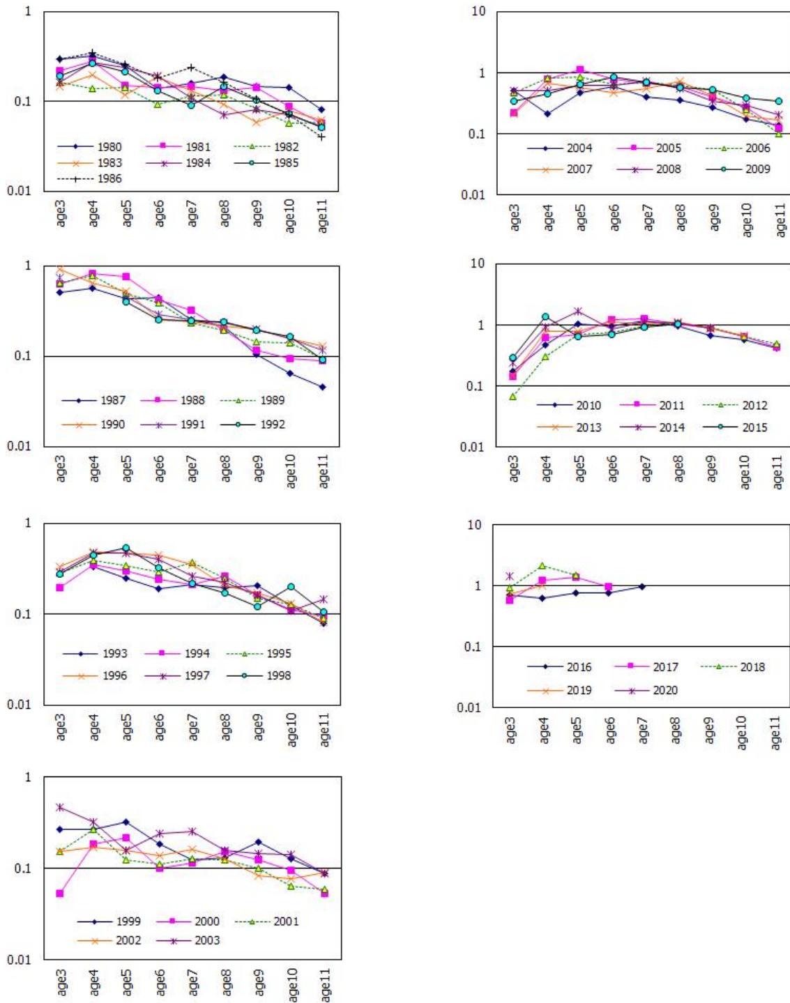
Fig. 1-3. Nominal CPUE of Japanese longline fishery by cohorts in log-scale.
