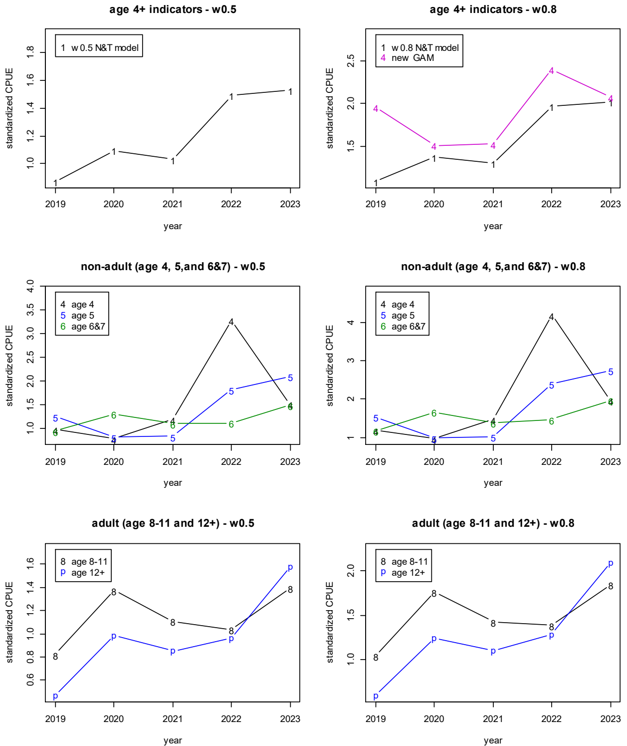
Fig. 5-2. Trends of CPUE-based indicators in recent years.
